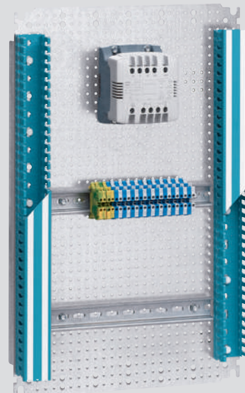
Fixing exemple on Lina 12.5 plate: - of a transformer with screws Cat.No 0 347 45 - of a rail - of Lina 25 cable ducting (p. 348)
