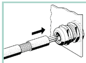
3. Insert cable to EMC spring
