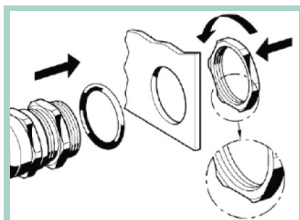
1. Tighten the cable gland
