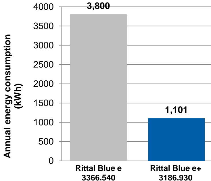
Projection of energy consumption per year*
