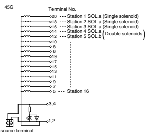
10GD/16GD Flat Ribbon Cable Type (PC Wiring)
