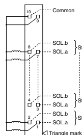
10PH/16PH Flat Ribbon Cable Type (10 pins)
