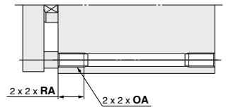
Both ends tapped (CQMA)
