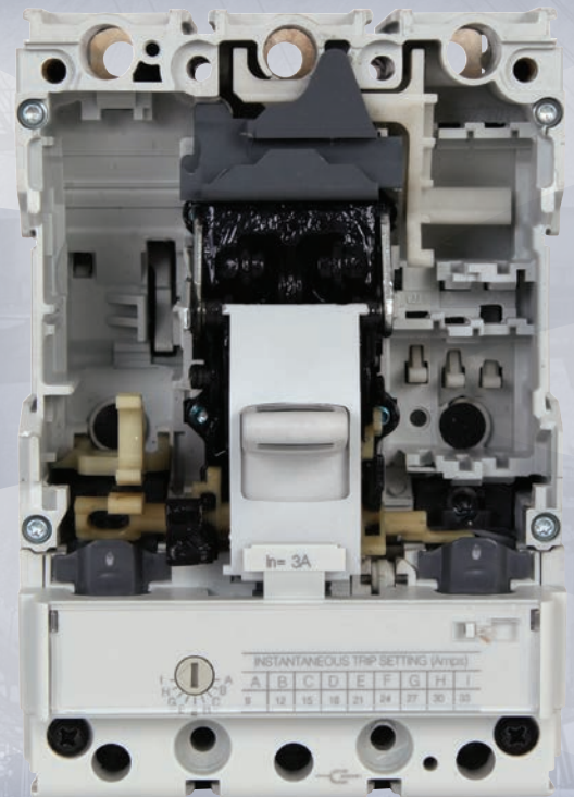
Shunt Trip/ Undervoltage Relay
