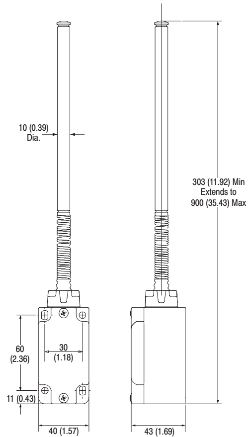
Telescopic Arm
