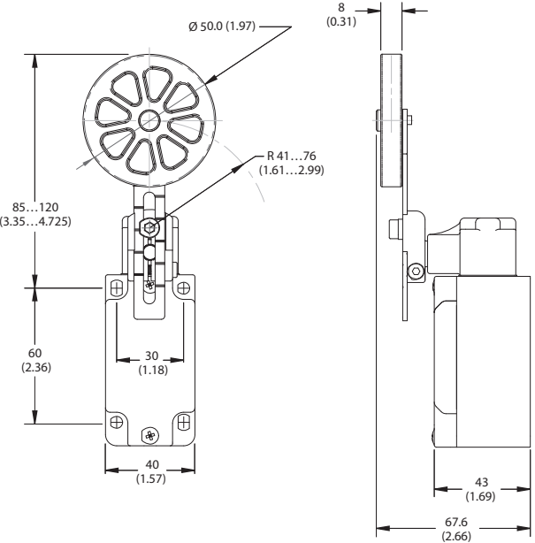
Adjustable Lever with Rubber Roller
