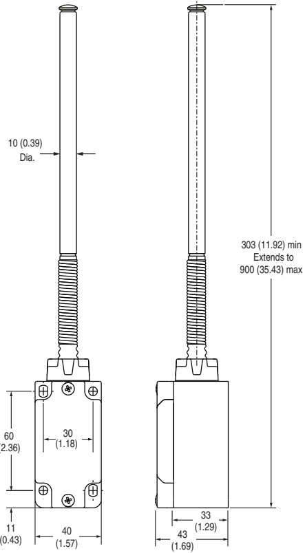
Telescopic Arm
