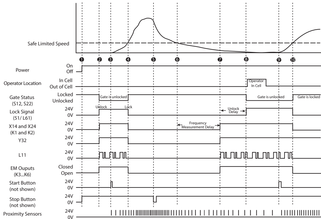
Figure 42 - Operational Sequence for Delayed Unlock with Auto Reset
