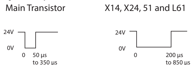
Figure 25 - Output Pulse Test Width
