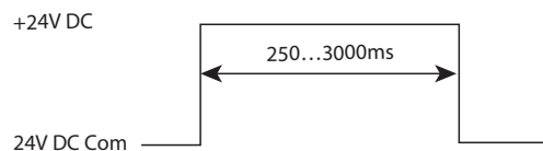
Figure 13 - Required Signal Duration
