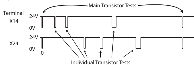
Figure 26 - Pulse Test Sequence
