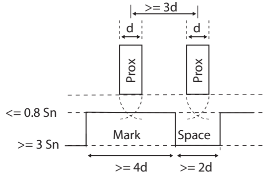
Figure 31 - Proximity Mark (Space Dimensions)
