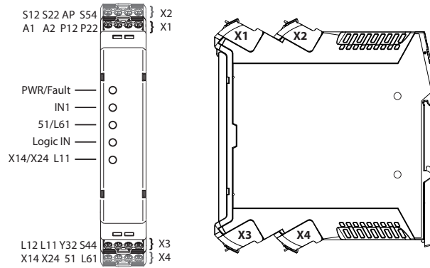
Figure 5 - Terminal Identification
