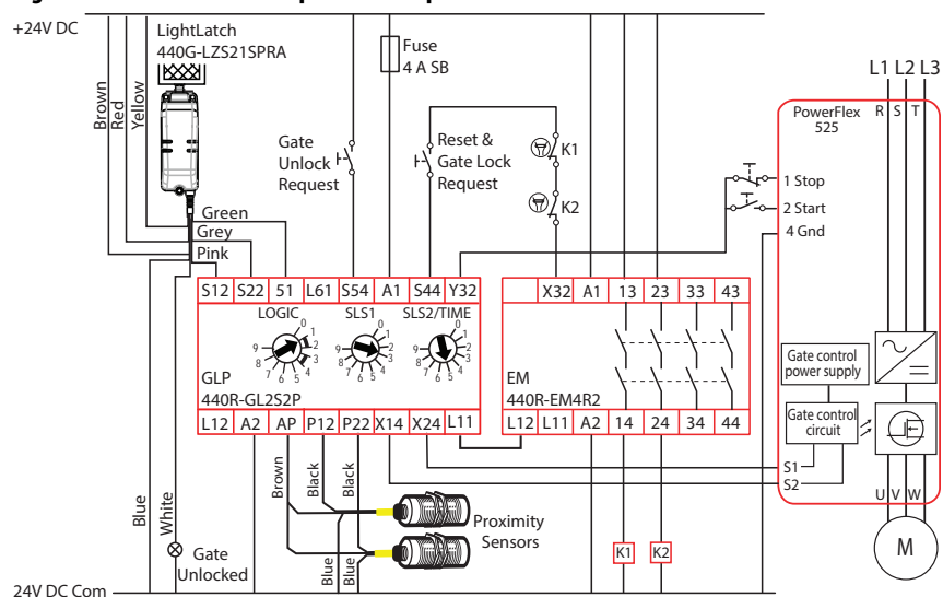
Figure 37 - Schematic for Stop Cat 1 Example
