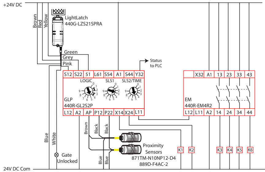
Figure 41 - Schematic for Delayed Unlock with Auto Reset
