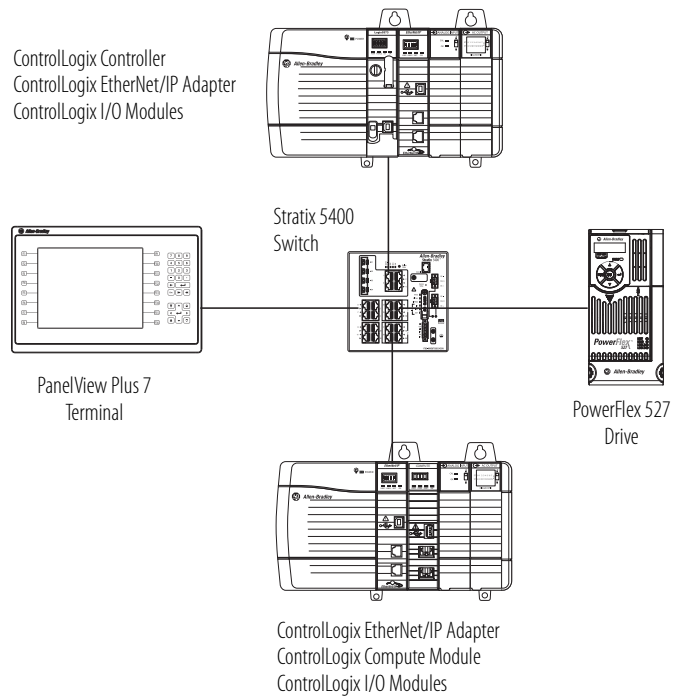
Compute Module Communication Over EtherNet/IP Network and Controller Chassis Backplane
