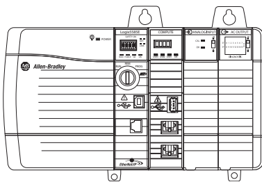
Compute Module Communication Over Backplane
