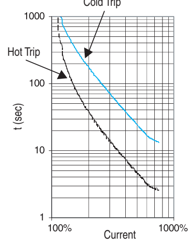
Trip Class 20
