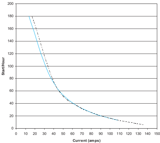
SMC-3 Starts per hour (108...135 A) 40C, 100% Duty Cycle, 20 sec, 350% (with standard fan)
