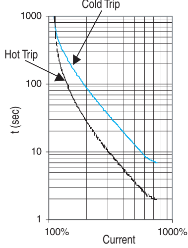
Trip Class 15
