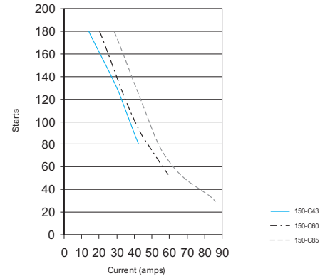
SMC-3 Starts per hour (43...85 A) 40C, 100% Duty Cycle, 20 sec, 350% (with standard fan)
