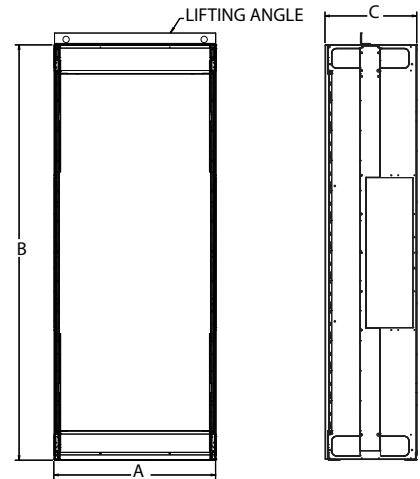
Figure 4 — Floor-Mount
