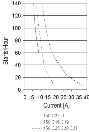
SMC-3 Starts per hour (3...37 A) 40 °C, 100% Duty Cycle, 10 s, 350% with Fan
