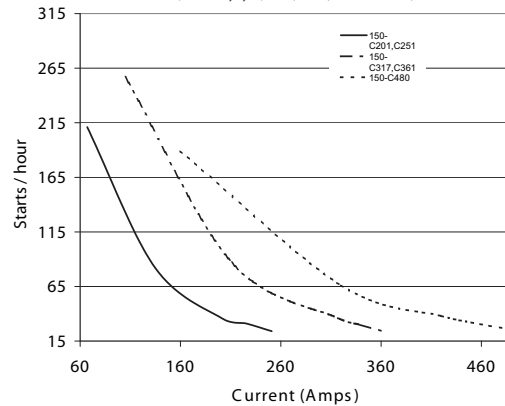
SMC-3 Starts per hour (201...480 A) 40C, 100% Duty Cycle, 20 sec, 350% (with standard fan)
