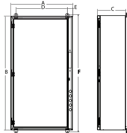
Figure 2 — Wall-Mount
