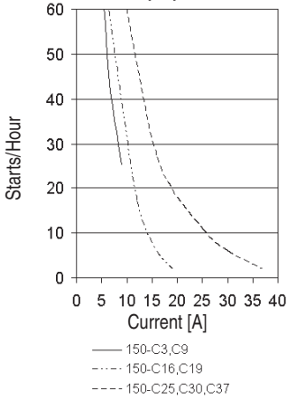
SMC-3 Starts per hour (3...37 A) 40 °C, 100% Duty Cycle, 10 s, 350% No Fan
