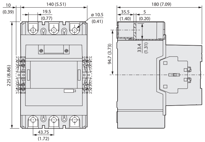
Figure 84 - 100-E265...100-E370 Contactors
