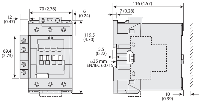
Figure 69 - 104-E80...104-E96 Reversing 3-Pole Contactors
