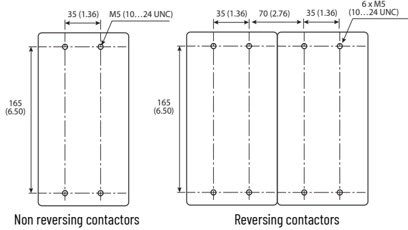
Figure 84 - 100-E265...100-E370 Contactors
