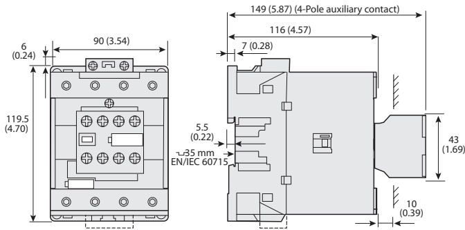
Figure 73 - 100-E80 4-Pole Contactors with Side-mounted Auxiliary Contact
