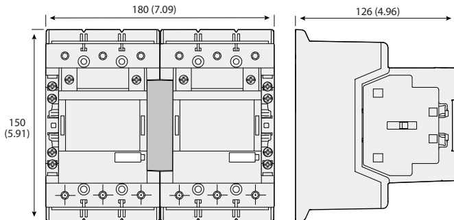
Figure 78 - 104-E116E..., 104-E146E... Reversing Contactors with Cat. No. 100-EM... Mechanical Interlock
