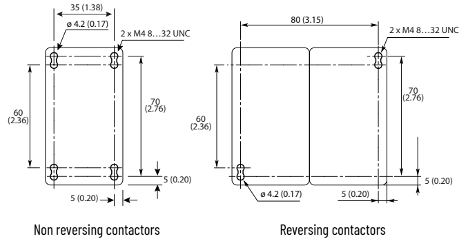
Figure 56 - Drilling Template for 26...38 A Contactors
