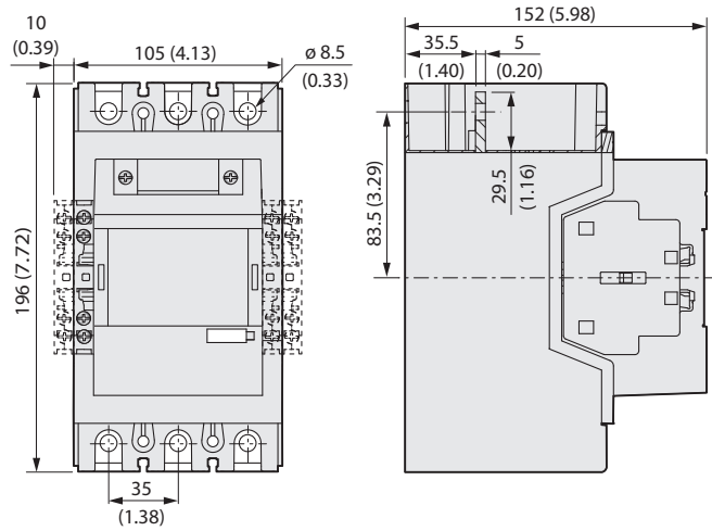
Figure 80 - 100-E190, 100-E205 Contactors
