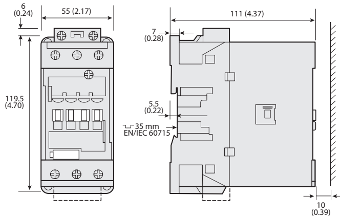
Figure 58 - 100-E40...100-E65 3-Pole Contactors with Front-mounted Auxiliary Contact
