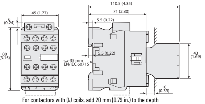
Figure 38 - 100-E09...100-E16 Contactors with Standard Coils and Side-mounted Auxiliary Contact
