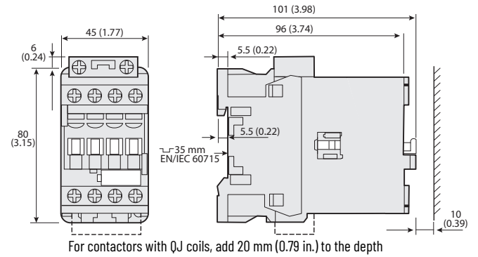
Figure 44 - 100-E26...100-E38 4-Pole Contactors with Standard Coils
