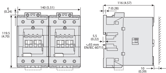
Figure 70 - Drilling Template for 80...96 A 3-Pole Contactors
