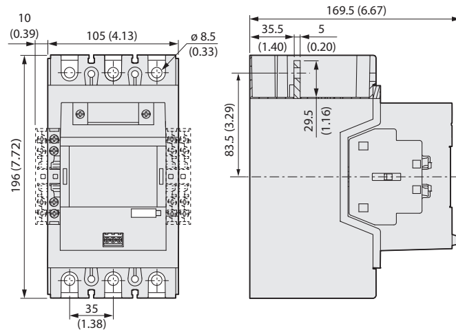
Figure 81 - 100-E190E, 100-E205E Contactors with PLC Input
