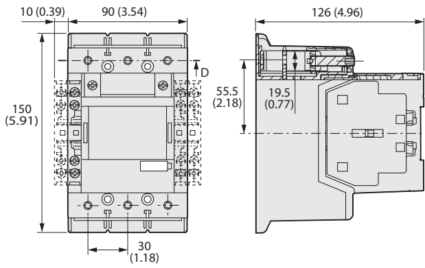
Figure 77 - 100-E116E..., 100-E146E... Contactors with PLC Input
