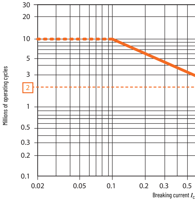
Figure 32 - Electrical durability for DC-13 utilization category - U_e \leq 250V
