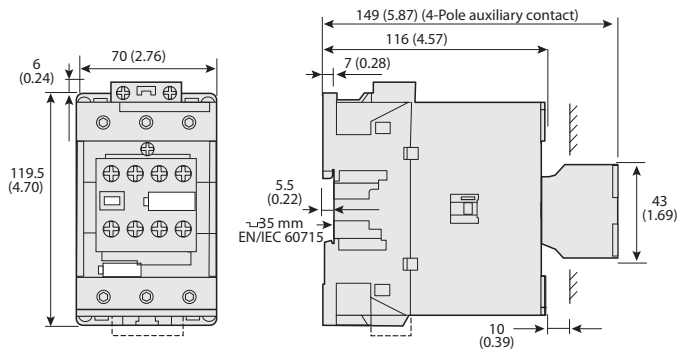
Figure 67 - 100-E80...100-E96 3-Pole Contactors with Front-mounted Auxiliary Contact
