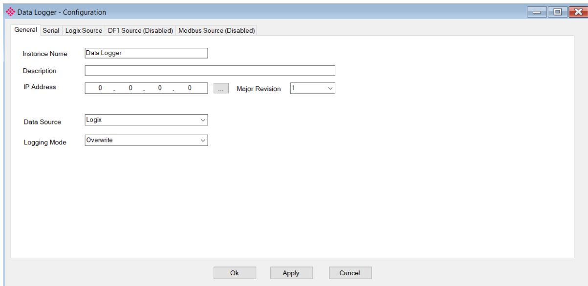
Figure 3.13 – PLX51-DL configuration
