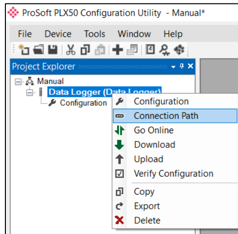
Figure 3.28 - Selecting Connection Path
