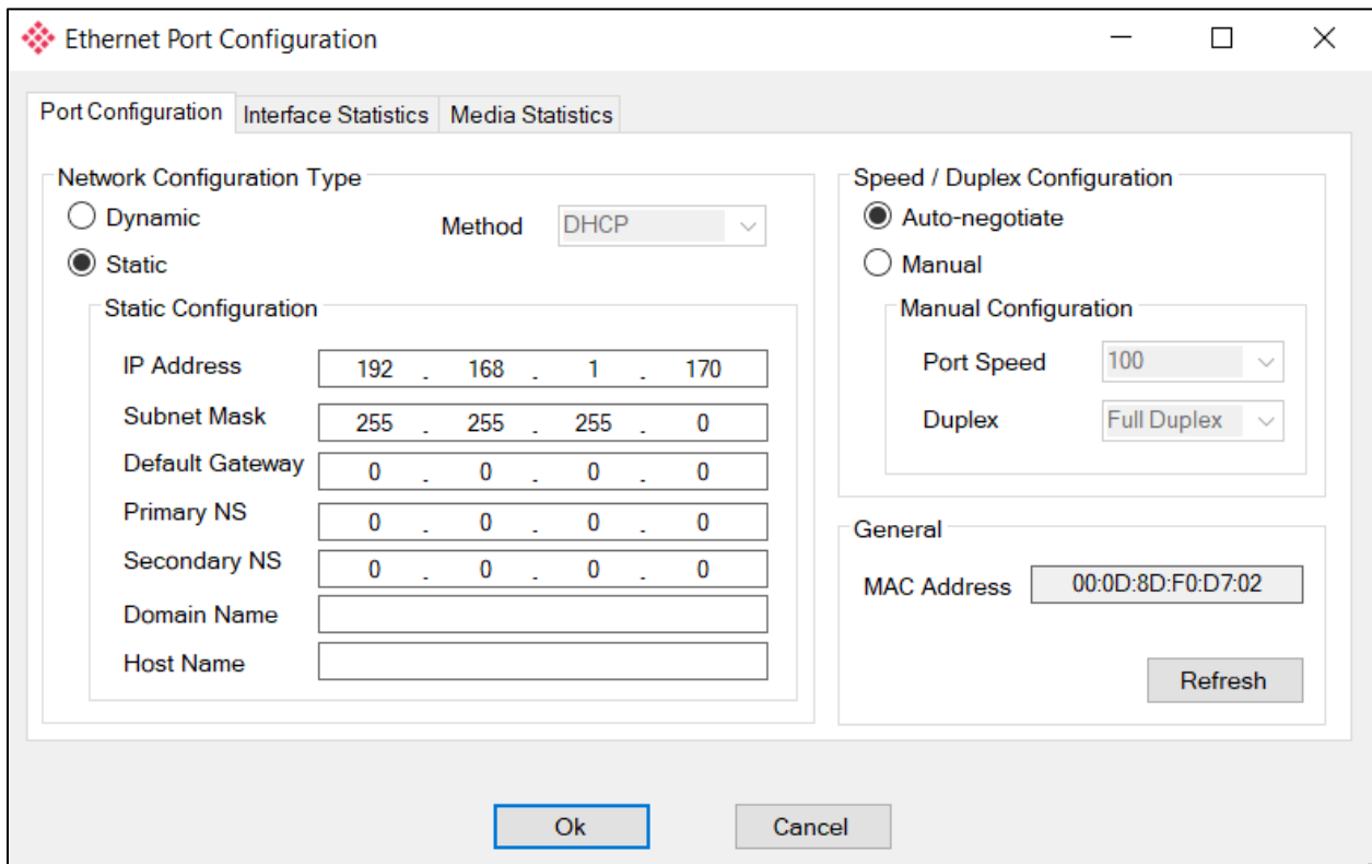
Figure 3.9. - Port Configuration
