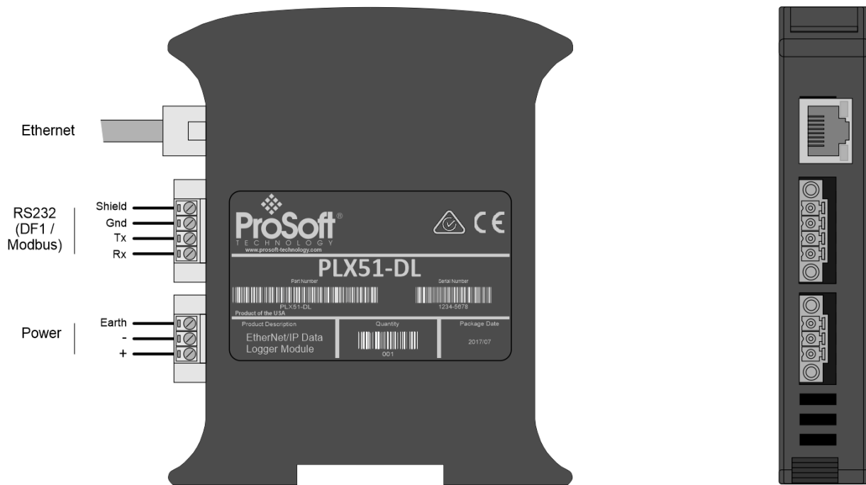
Figure 2.1. – Data Logger side and bottom view
