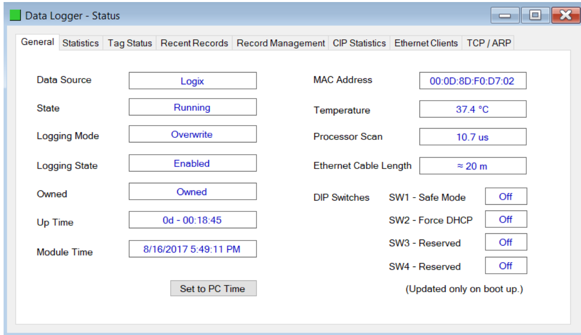
Figure 6.4 - Status monitoring - General
