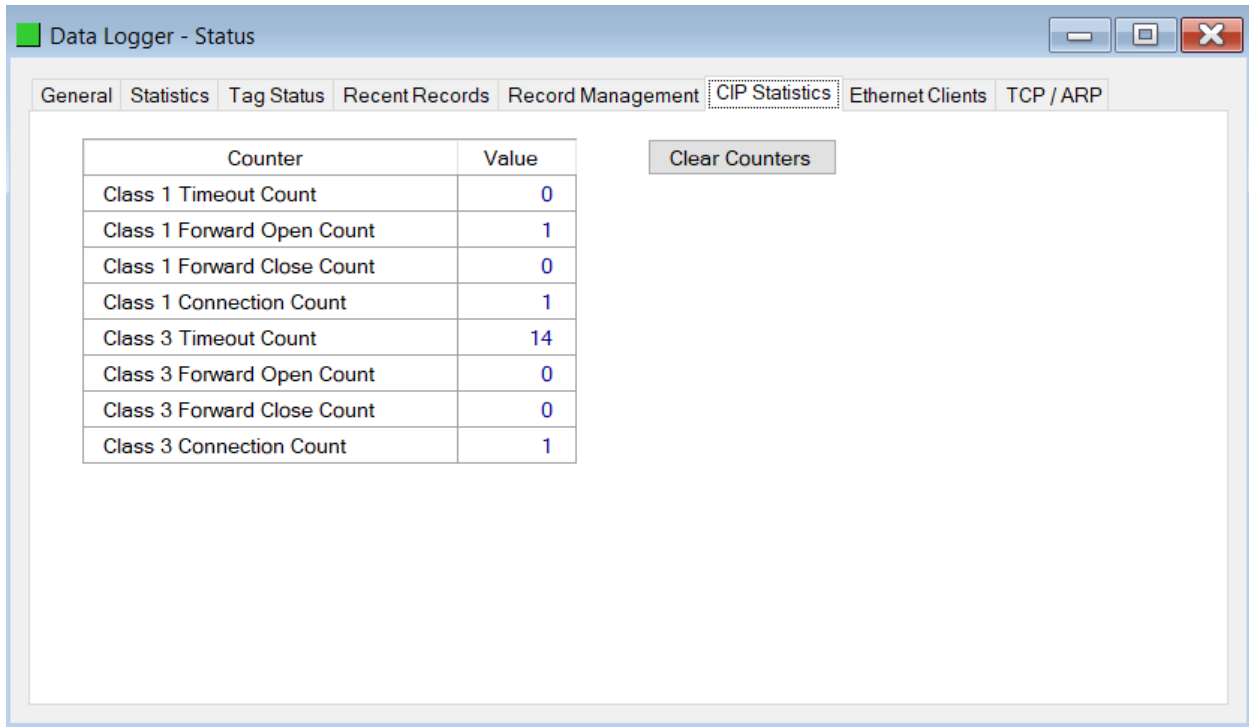
Figure 6.9 – CIP Statistics
