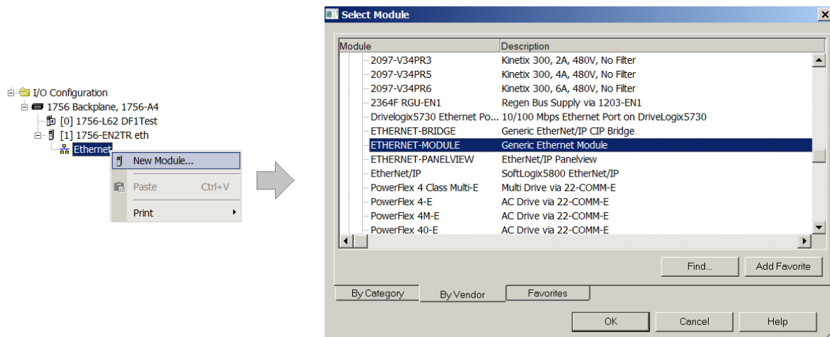
Figure 5.1 - Add a Generic Ethernet Module in RSLogix 5000
