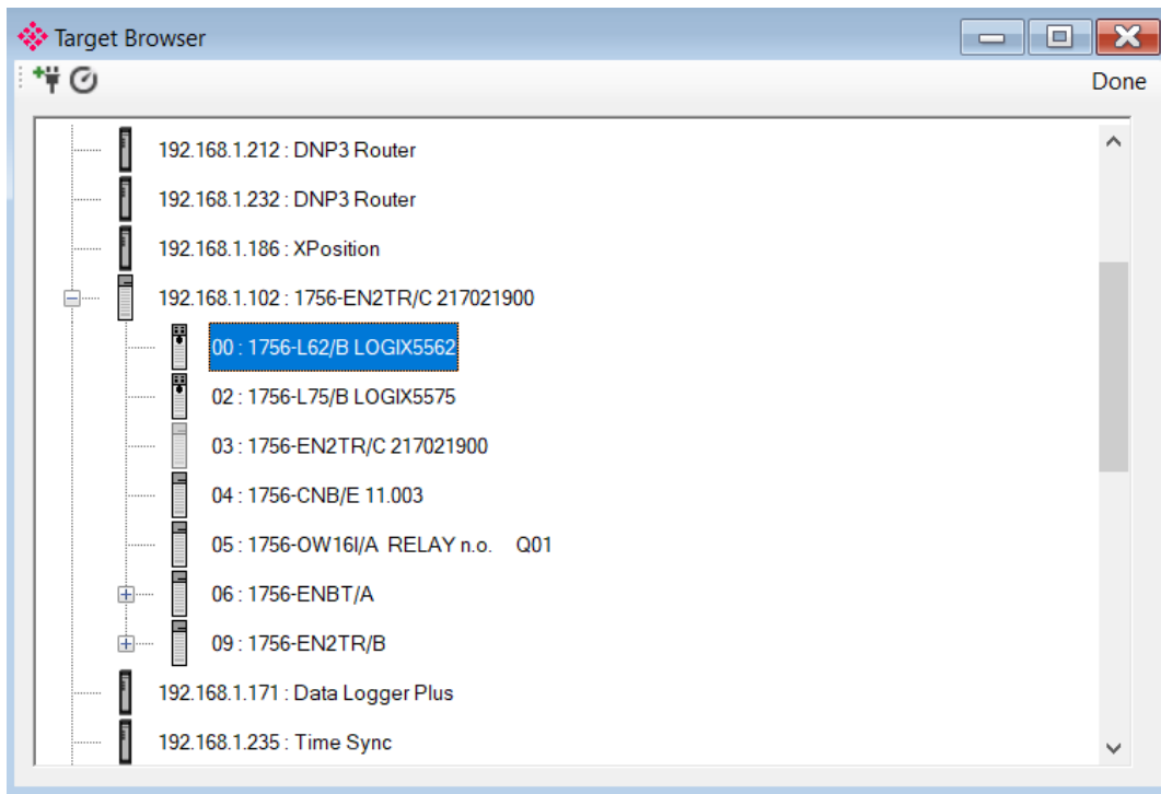
Figure 3.21 – Target Browser Window
