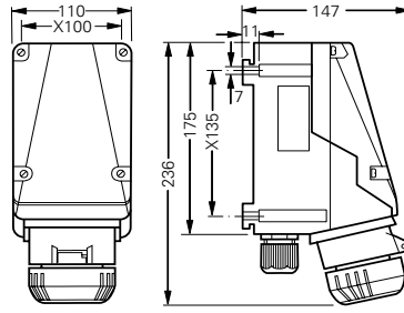
Wall socket 4/5-pole
